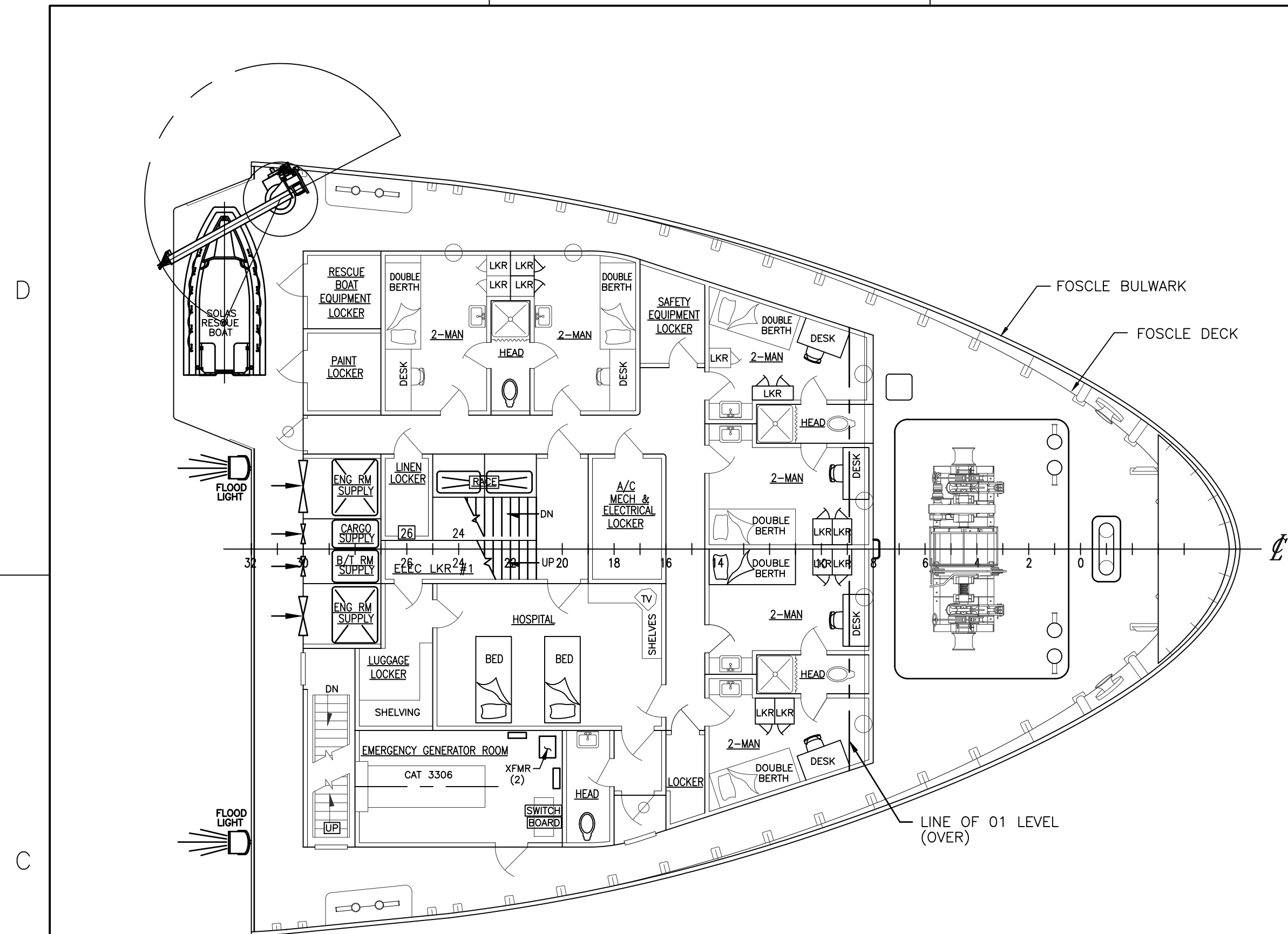
FOCSLE DECK 32'-0" ABOVE BASELINE
