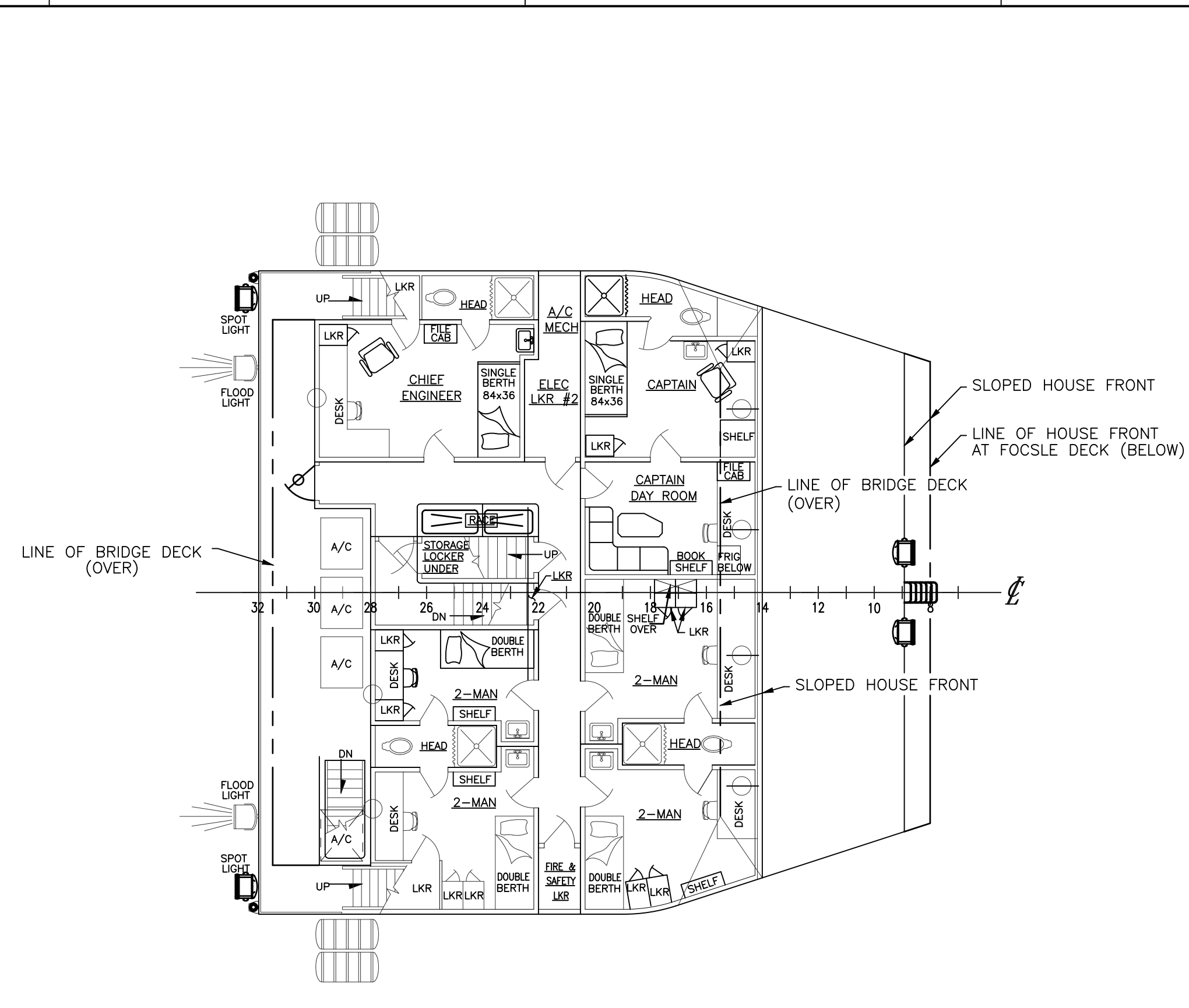
01 DECK 41'-7 5/8" ABOVE BASELINE
