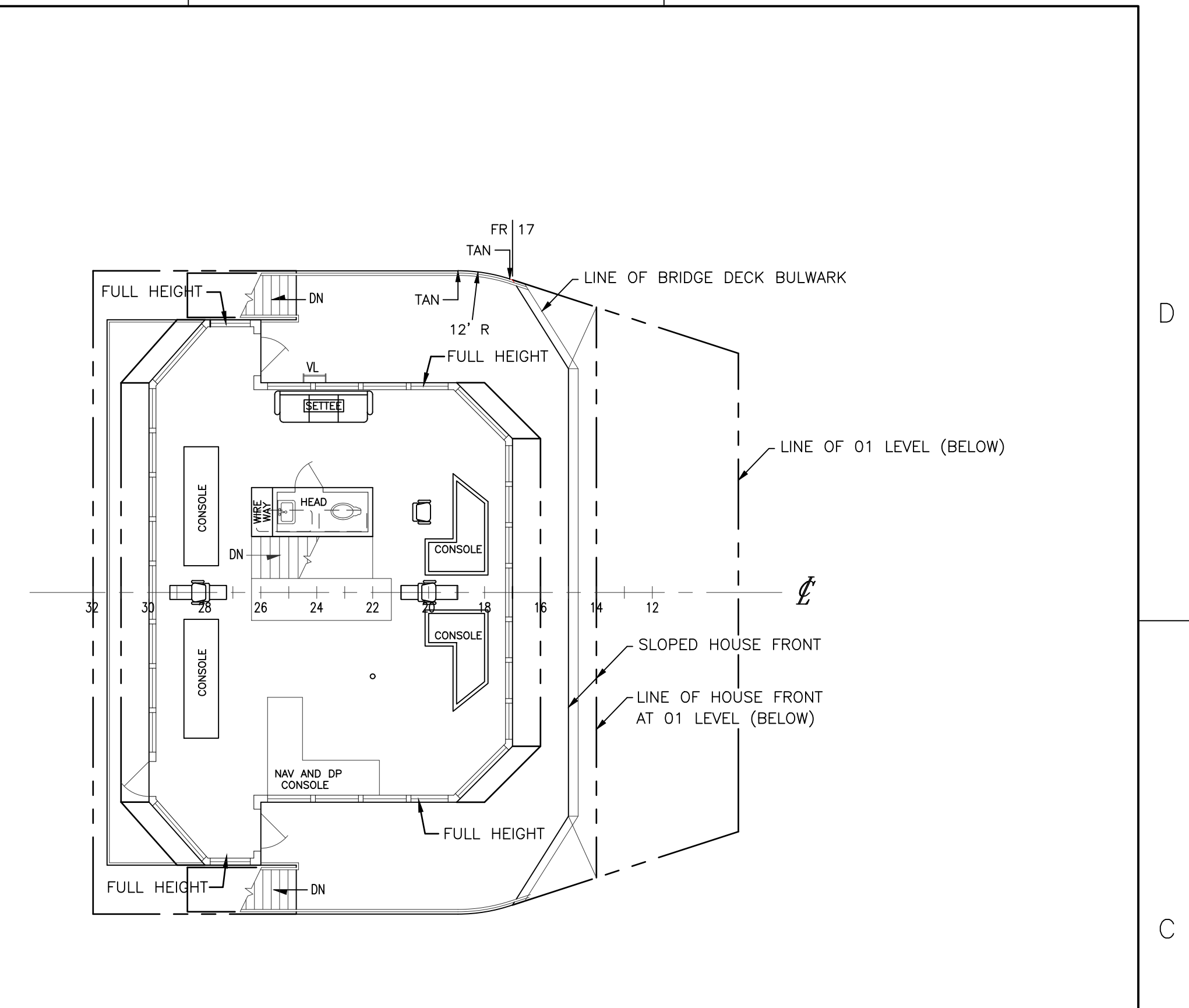
BRIDGE DECK 51'-7 5/8" ABOVE BASELINE
